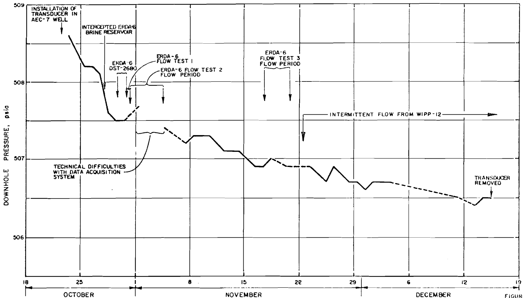
FIGURE H-16 PRESSURE IN OBSERVATION WELL AEC-7 DURING TESTING OF ERDA-6 AND WIPP-12 BRINE RESERVOIRS PREPARED FOR WESTINGHOUSE ELECTRIC CORPORATION ALBUQUERQUE, NEW MEXICO
