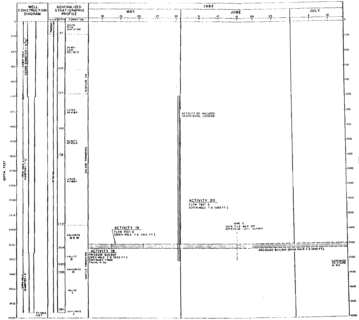
FIGURE H-2b WIPP-12 CONTINUATION OF TIME-VERSUS-DEPTH ACTIVITY SUMMARY PREPARED FOR WESTINGHOUSE ELECTRIC CORPORATION ALBUQUERQUE, NEW MEXICO
