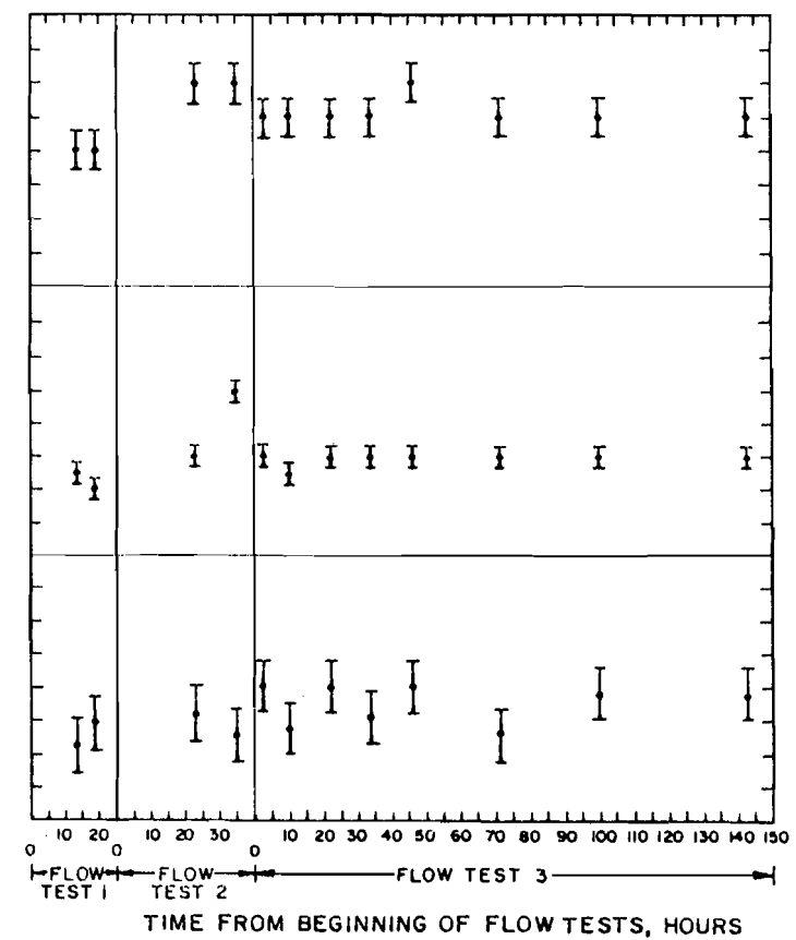
FIGURE C-1d CONCENTRATION OF SELECTED PARAMETERS VERSUS FLOW RATE AND FLOW TIME WIPP-12
