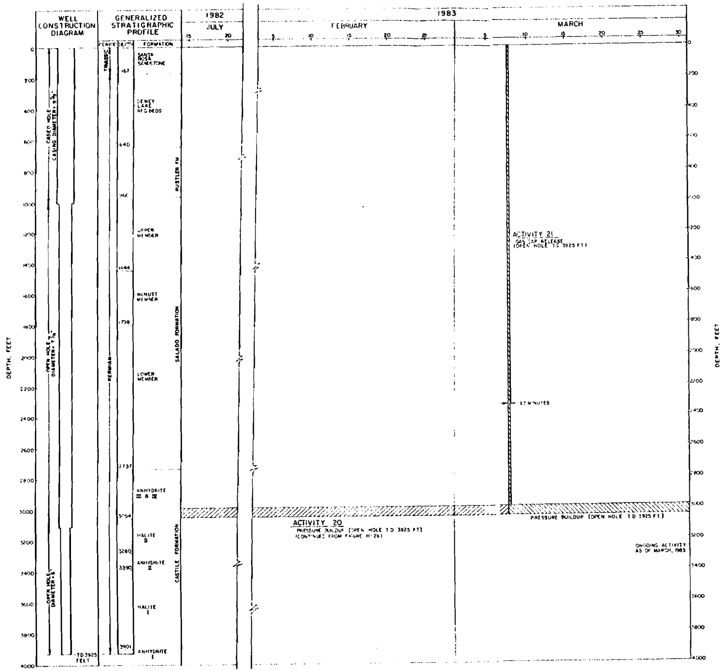
FIGURE H-2c WIPP-12 CONTINUATION OF TIME-VERSUS-DEPTH ACTIVITY SUMMARY PREPARED FOR WESTINGHOUSE ELECTRIC CORPORATION ALBUQUERQUE, NEW MEXICO D'APOLONIA
