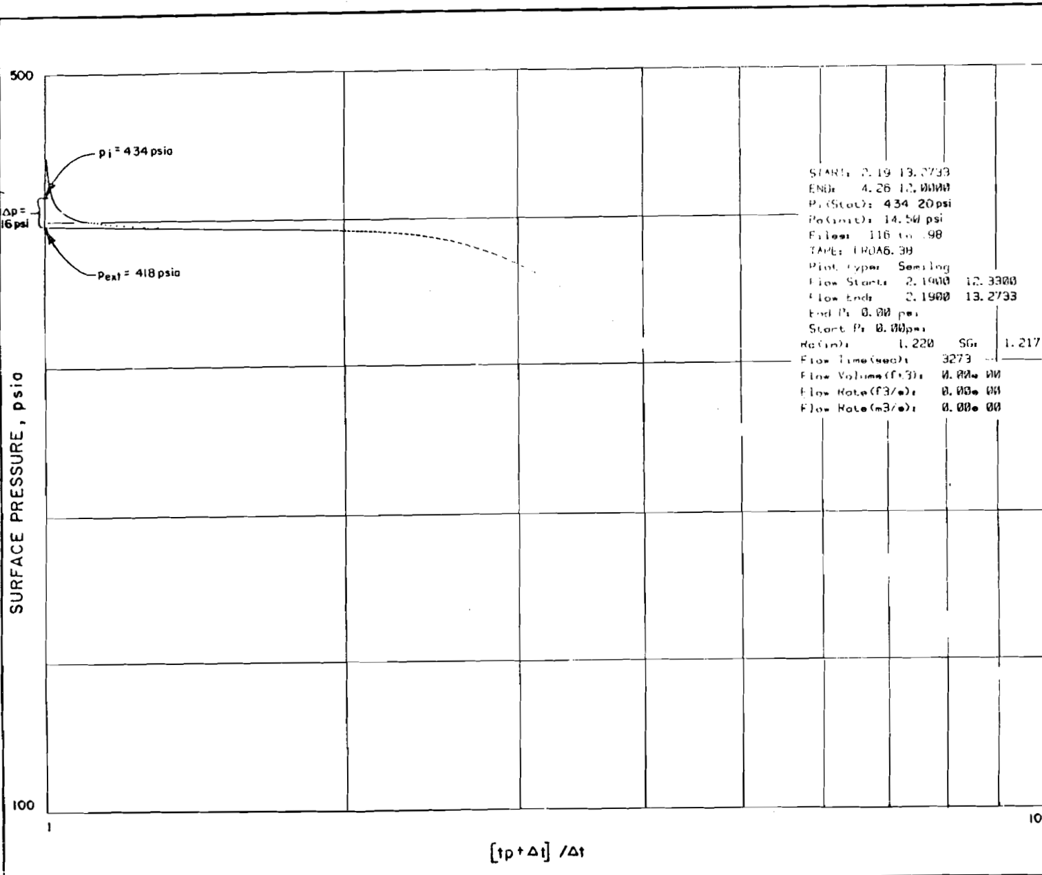
FIGURE H-7 HORNER PLOT OF ERDA-6/ BOP CHANGE/ BUILDUP PERIOD DATA PREPARED FOR WESTINGHOUSE ELECTRIC CORPORATION ALBUQUERQUE, NEW MEXICO
