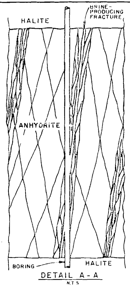
FIGURE G-13 SCHEMATIC OF BRINE RESERVOIR FORMATION PREPARED FOR WESTINGHOUSE ELECTRIC CORPORATION ALBUQUERQUE, NEW MEXICO IDAHO POWER COMPANY
