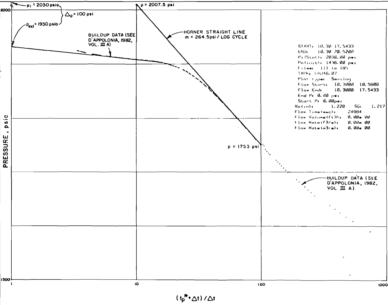
FIGURE H-6 HORNER PLOT OF ERDA-6/ FLOW TEST 1/ BUILDUP PERIOD DATA PREPARED FOR WESTINGHOUSE ELECTRIC CORPORATION ALBUQUERQUE, NEW MEXICO H D'APPOLONIA
